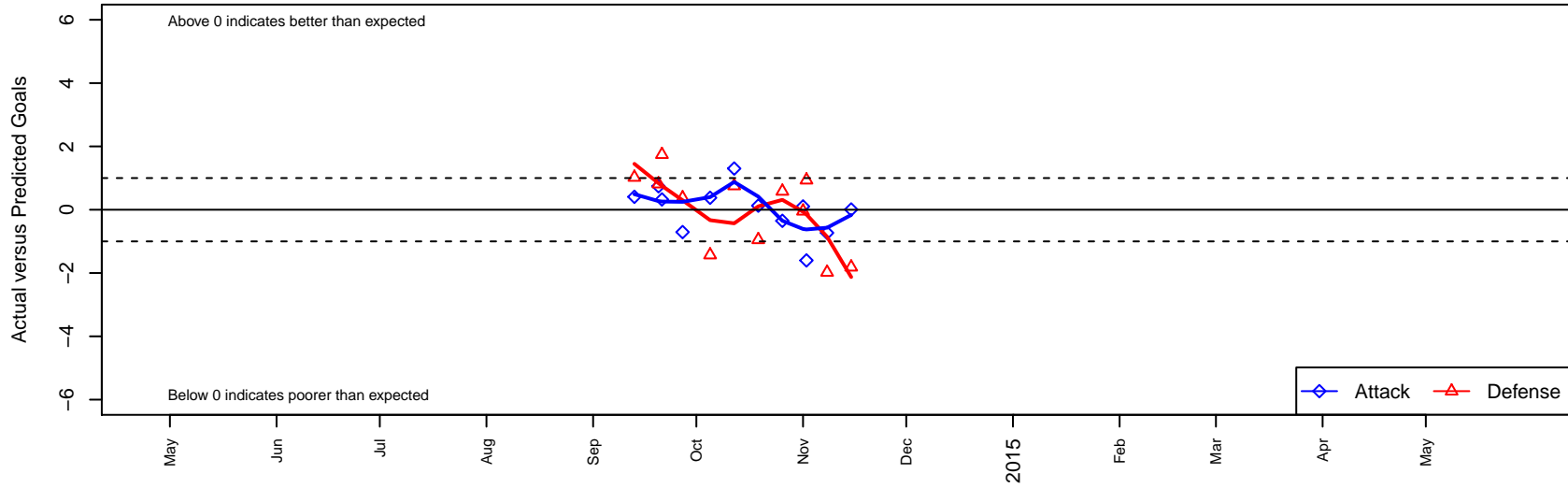
Strikers FC Mission Viego B97 Dots are actual minus expected GF (blue circles) and GA (red triangles). Blue line is smoothed change in attack strength. Red is smoothed change in defense strength.
